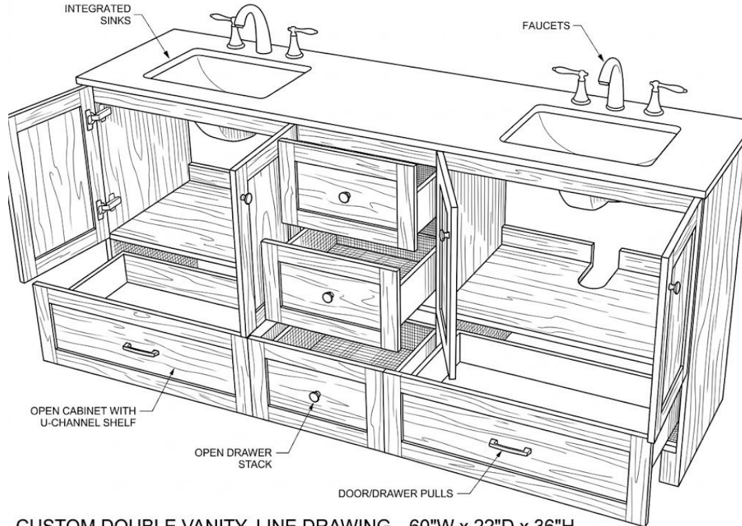
CUSTOM DOUBLE VANITY LINE DRAWING - 60"W x 22"D x 36"H
